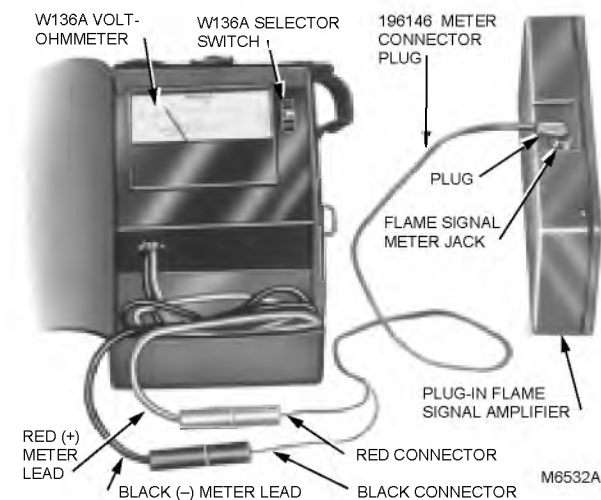
Fig. 11—Measuring microamp flame signal.
